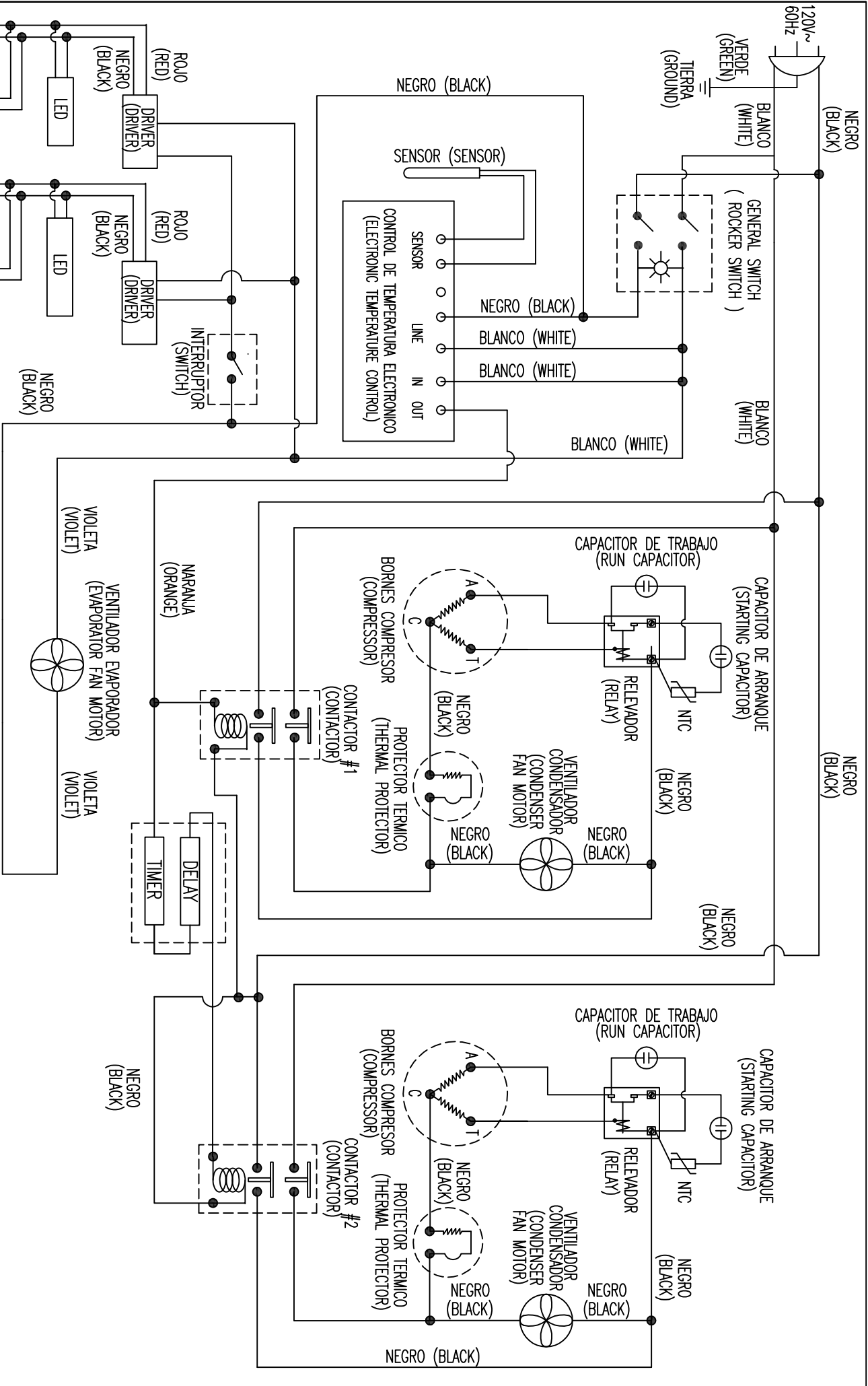
DIAGRAMA ELECTRICO (ELECTRIC DIAGRAM) VMHCSL-18
